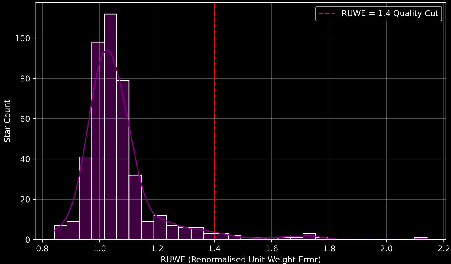
GAPOGEE DR17 Field [184+00] RUWE Distribution (n= 435)
