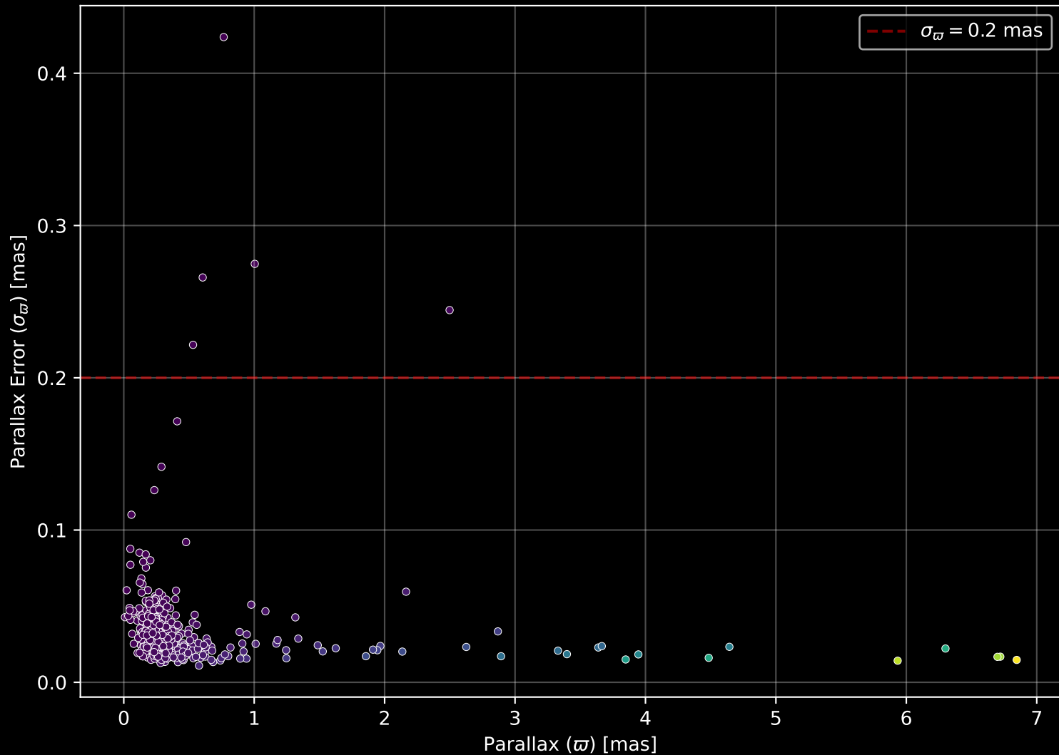
APOGEE DR17 Field: [184+00] Parallax Quality (n= 440)
