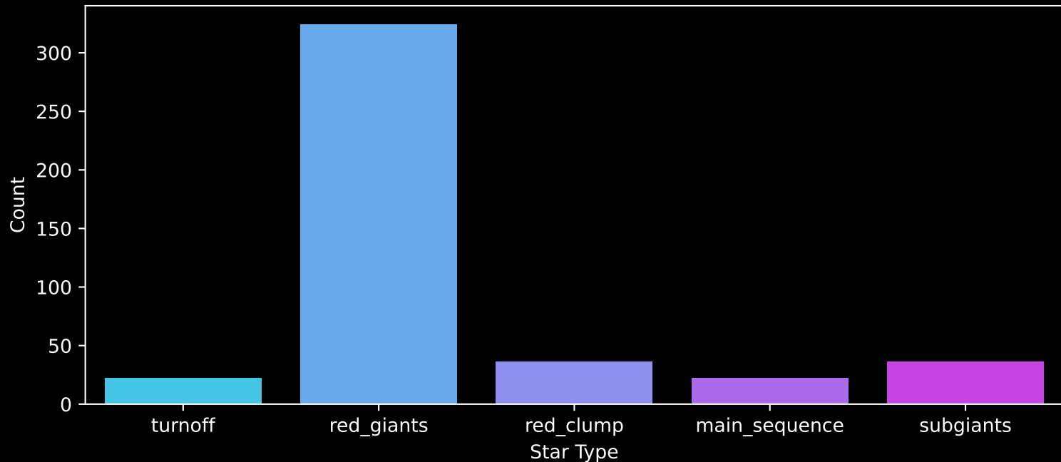
APOGEE DR17 Field: [184+00] Count plot of Star Type
