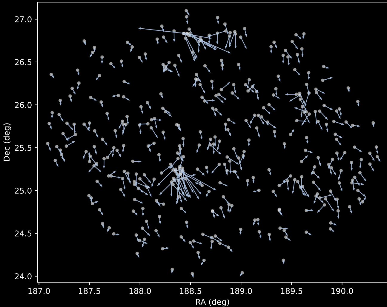
APOGEE DR17 Cluster 1 Proper Motion Vectors (n=364)
