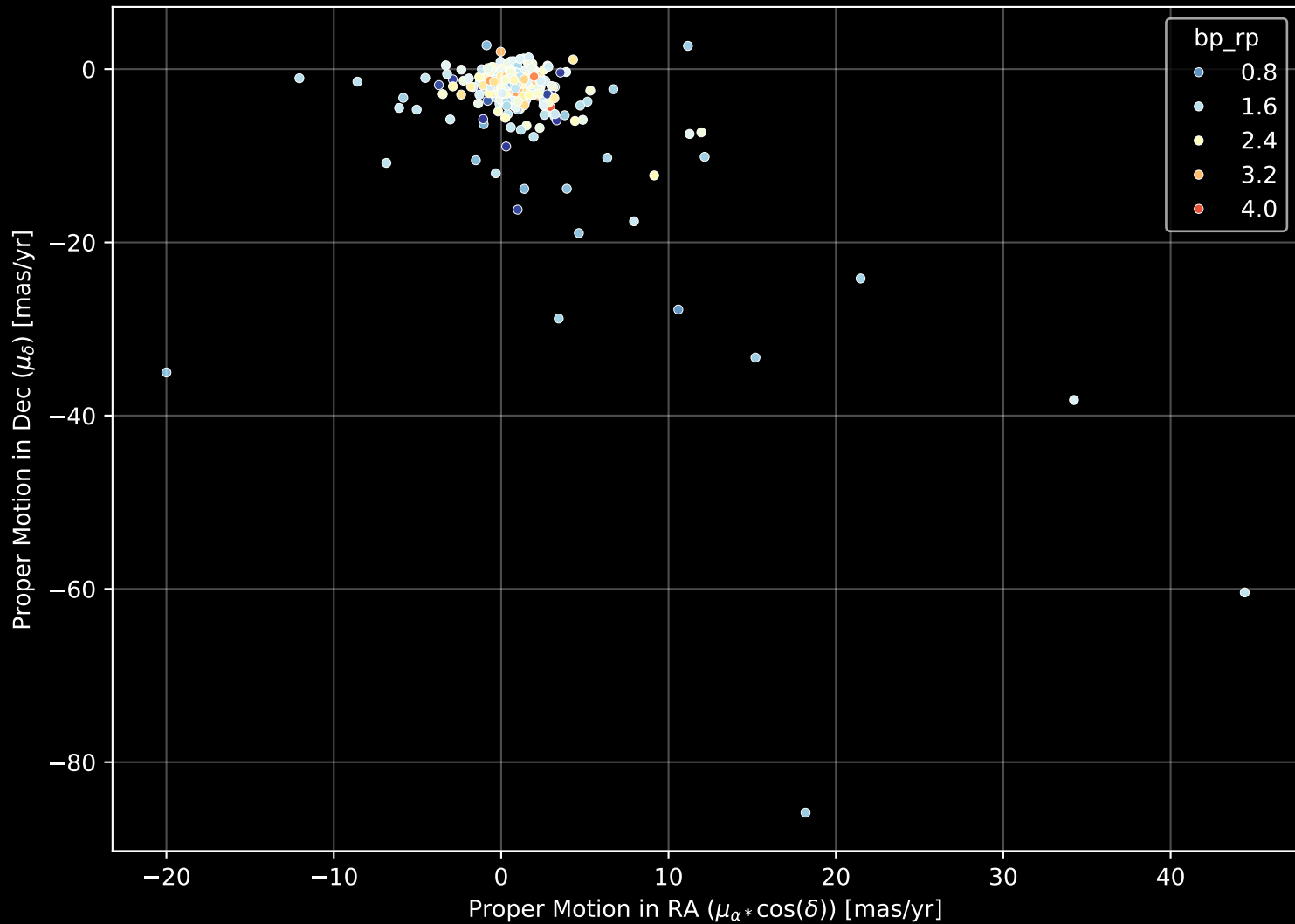
APOGEE DR17 Field: [184+00] Proper Motion Diagram (n= 440)
