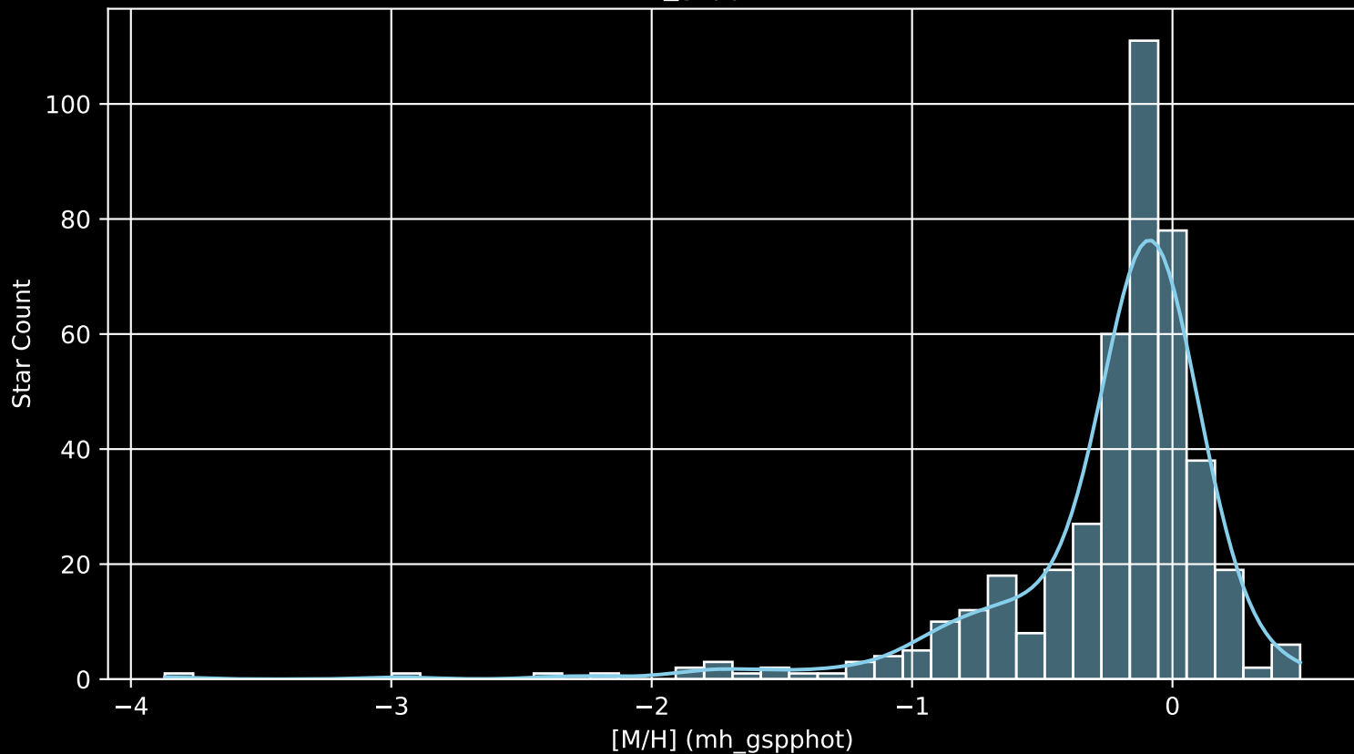
APOGEE DR17 Field: [184+00 [M/H] (mh_gspphot) (n= 434)
